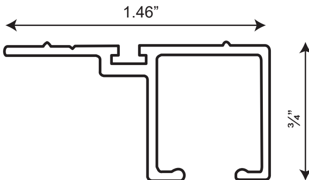
Ceiling Mount Squared 0.75" Model # BP658
